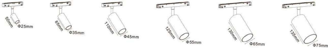
RL-TL1026-3W RL-TL1026-5W RL-TL1026-7W RL-TL1026-10W RL-TL1026-15W RL-TL1026-20/23W
