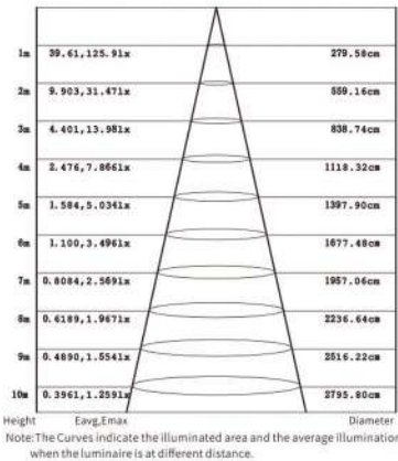
Luminaire effective average illumination diagram
